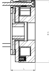
SECTION AA SCALE 1:1
